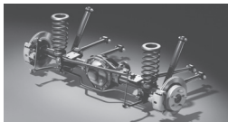
Segment exclusive** five-link coil spring rear suspension
